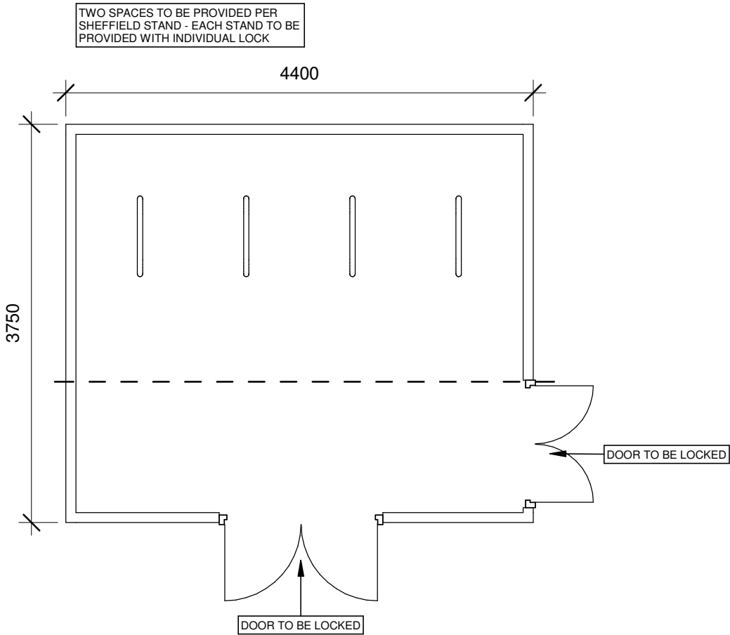
Cycle Store Layout 1 : 50
